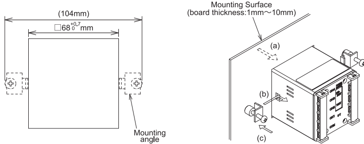
Mounting Dimensions Diagram
