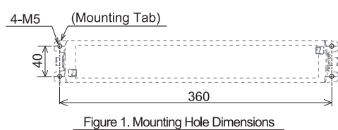
Figure 1. Mounting Hole Dimensions
